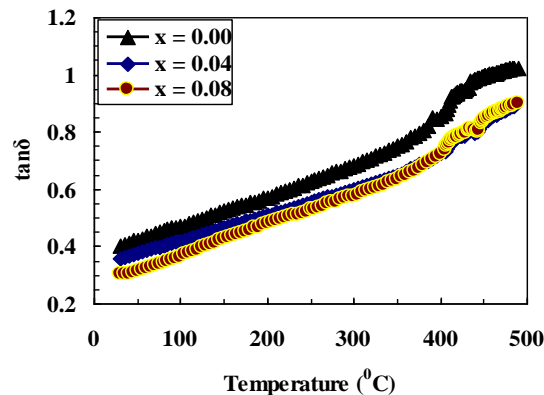
Fig. 2. Temperature dependence of loss tangent of Sr-hexaferrites of compositions (SrO)_{1-x}(La_2O_3)_x \cdot 5.7Fe_2O_3 , where x = 0.00, 0.04, 0.08 sintered at 1235°C in air for 2 hours.
